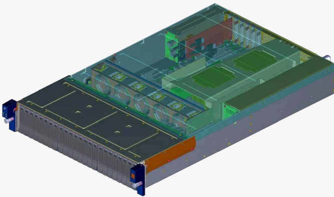
Figure 2: Samsung NVMe Reference Design
