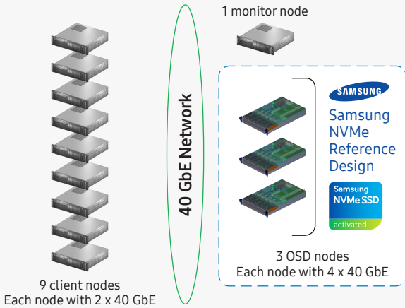
Figure 3: Samsung-Ceph Reference Architecture cluster
